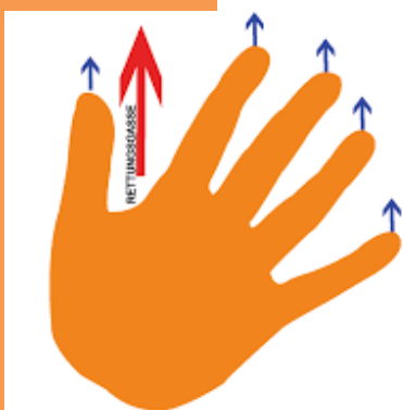
Rechte- Hand- Regel
